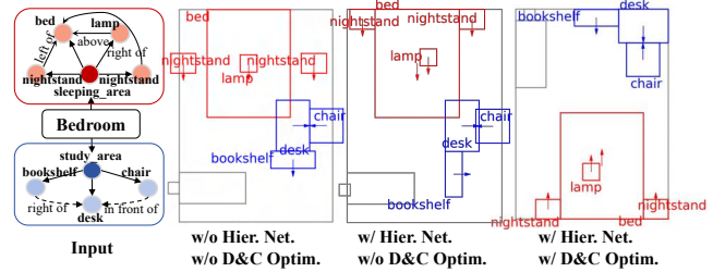
Figure 5: Topview visualizations of the ablation study.
